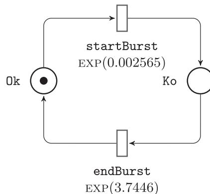
Fig. 1. STPN model of communication failures due to burst noise (time expressed in s).
