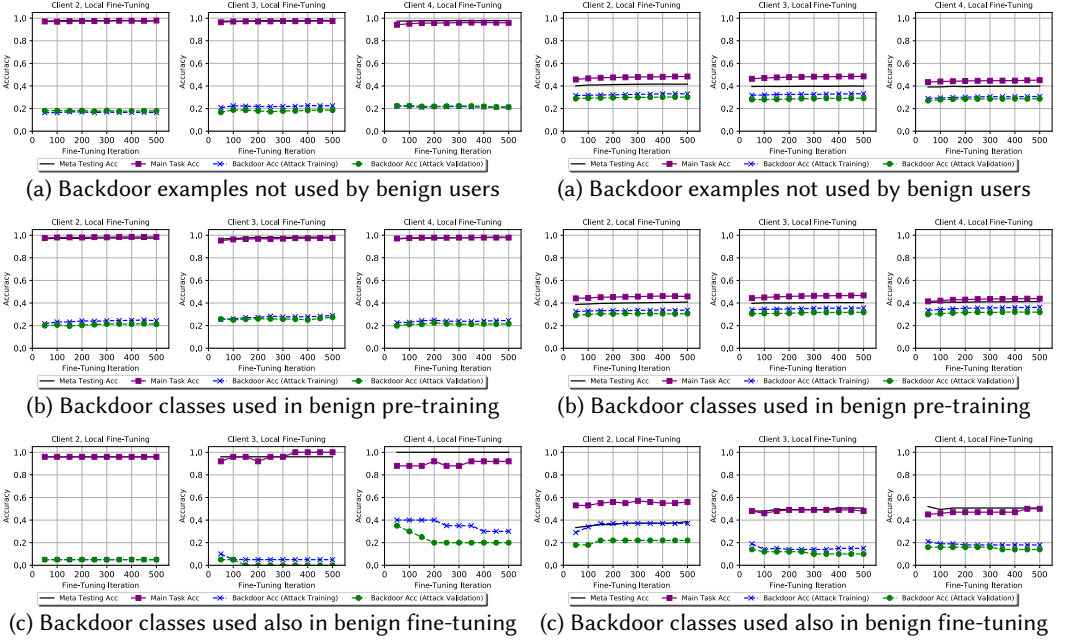
Fig. 22. Benign fine-tuning ( \eta = 0.001, \delta = 0.3 ) after attacks on Omniglot
