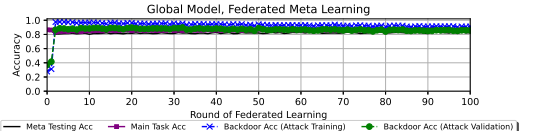
(b) Backdoor classes used in benign pre-training
